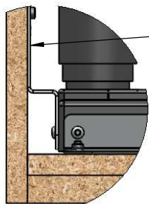
DETAIL A SCALE 1 : 3
