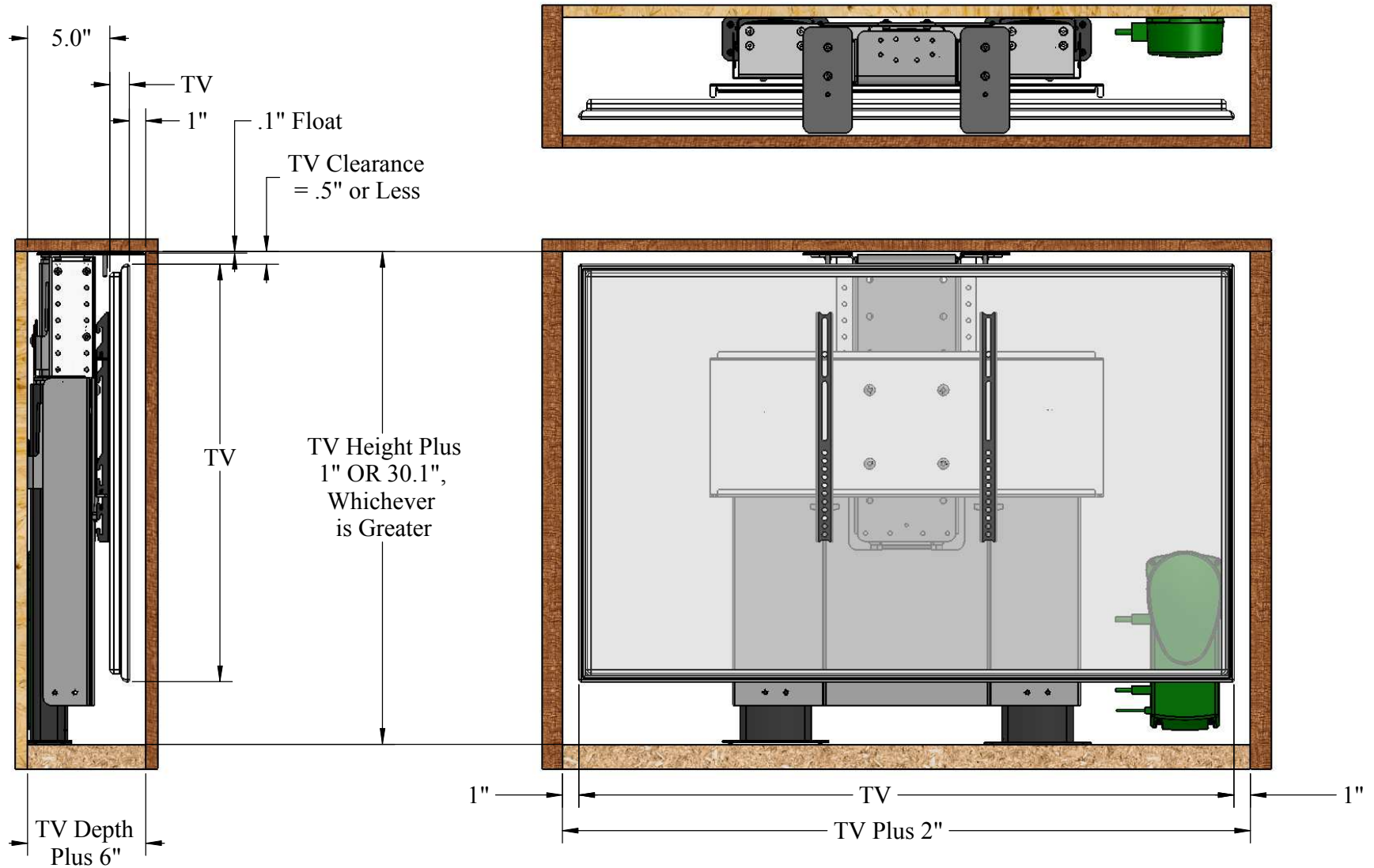
Model L-53 Installation Dimensions: Standard Configuration
